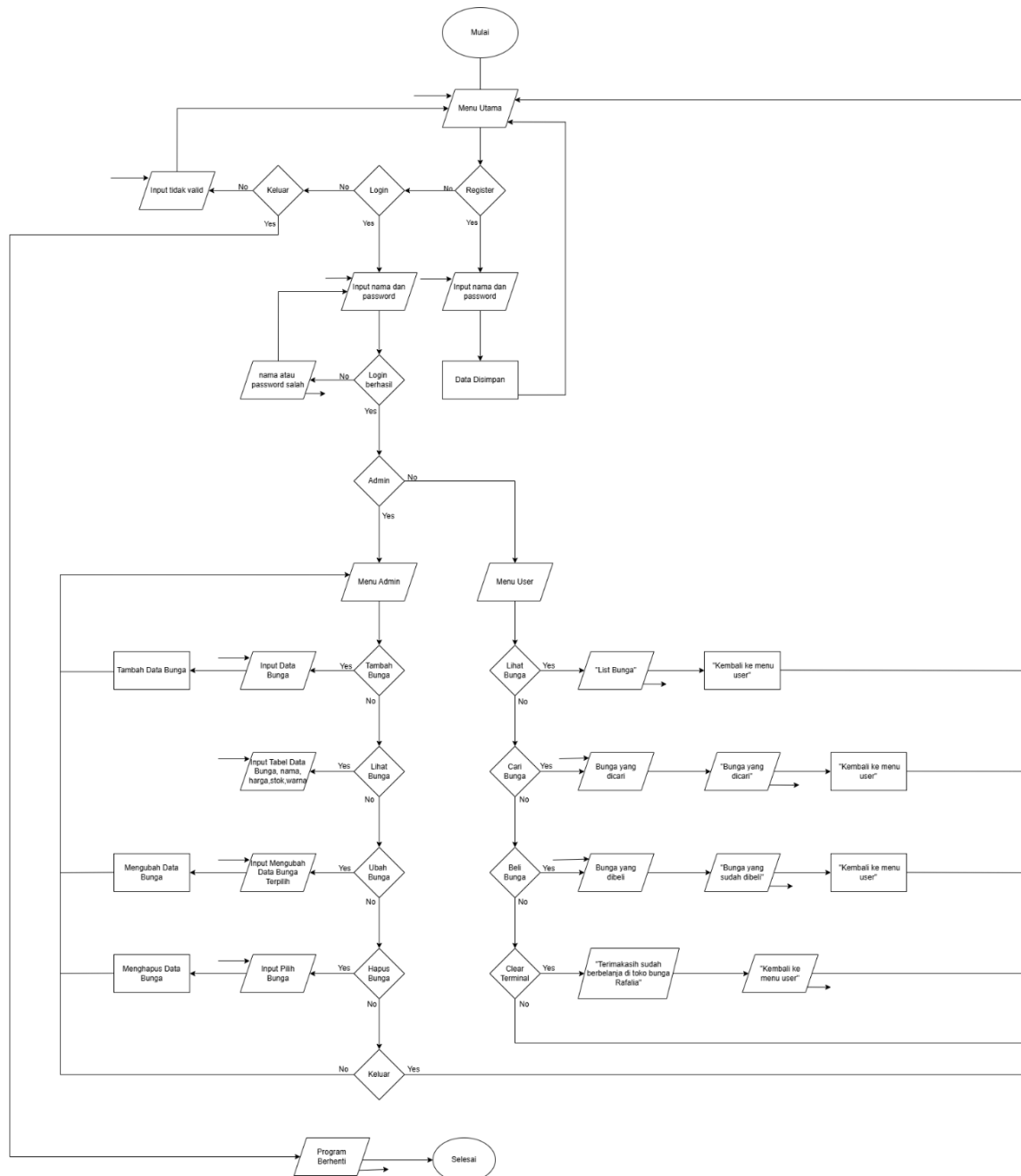
Gambar 1.1 Flowchart
